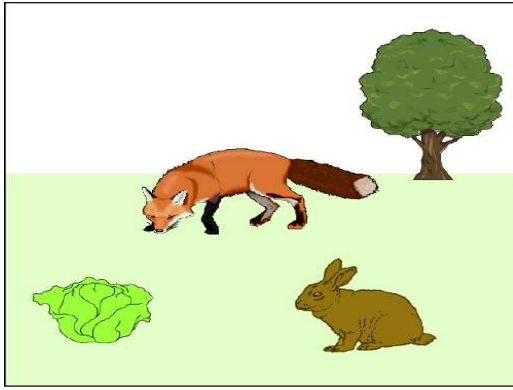
Figure 1: Selectional Restrictions.
