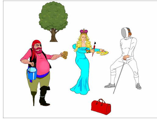
Figure 2: Depicted Events.
