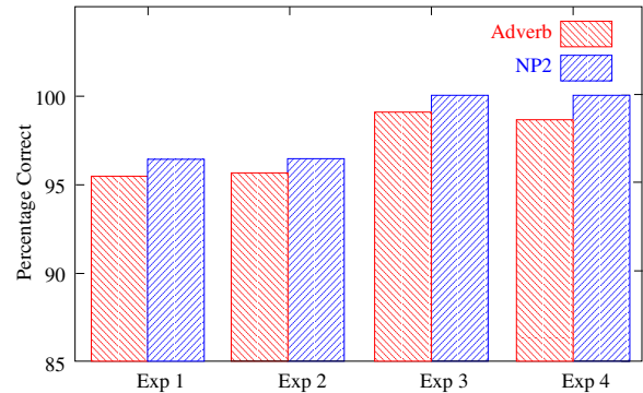
Figure 4: Results.
